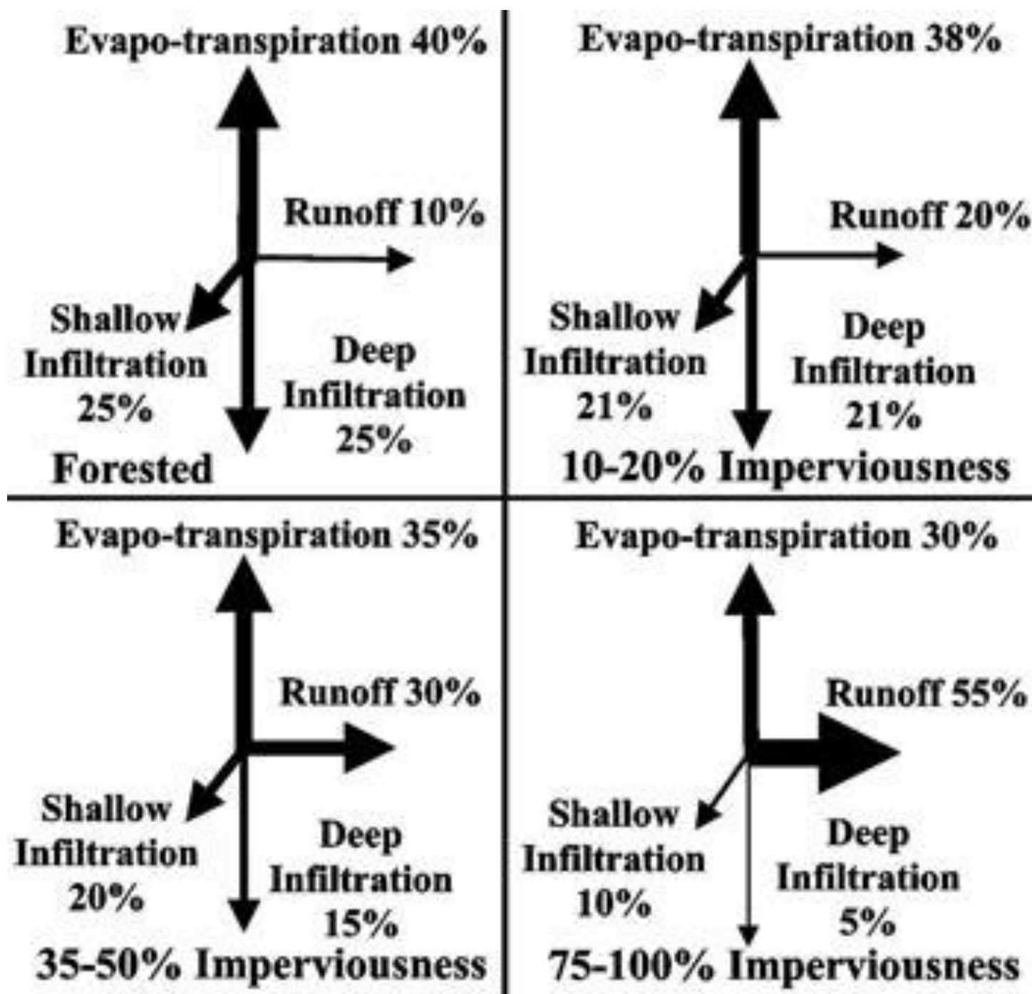
Figure 16. The shift in relative hydrologic flow in increasingly impervious watersheds. Note the large increase in stormwater runoff as imperviousness increases, at the expense of infiltration. From Paul MJ & Meyer JL. 2001. The ecology of urban streams . Annual Review of Ecology & Systematics 32:333-365. © 2001 by Annual Reviews. Reprinted with permission. https://www.epa.gov/caddis/urbanization-stormwater-runoff
